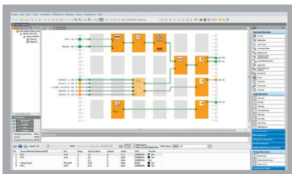
The state of the inputs and outputs of the configured elements and the connections between the elements are displayed.
