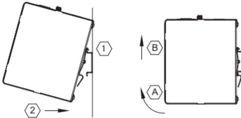
Figure 4: DIN-rail installation
