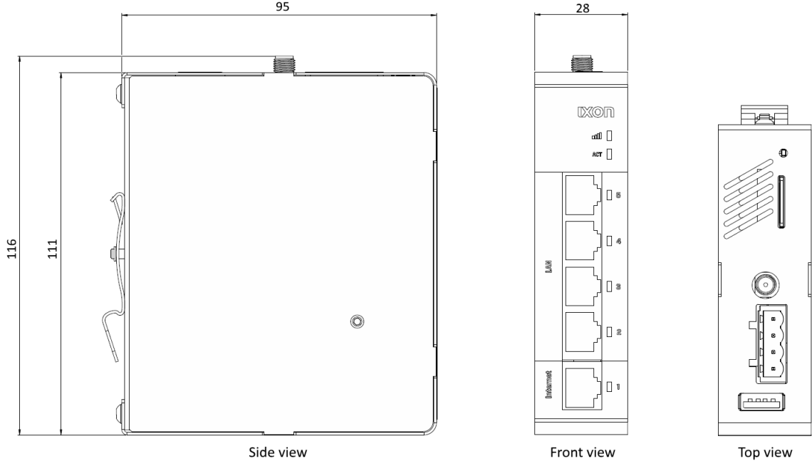
Figure 3: IXrouter3 dimensions
