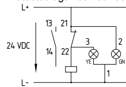
Z/T 335, 355 with LED (ordering suffix G24)
