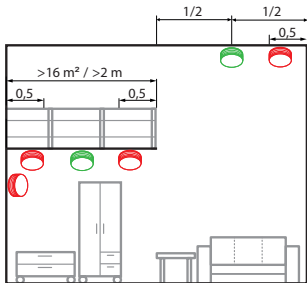
Fig. 7 Rooms with a platform or gallery
